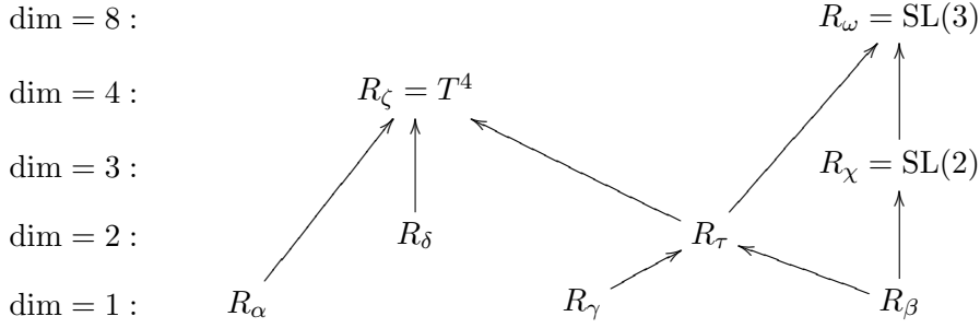
FIGURE 1. The adjacencies of connected reductive subgroups with Z_R^{ss} \neq \emptyset
