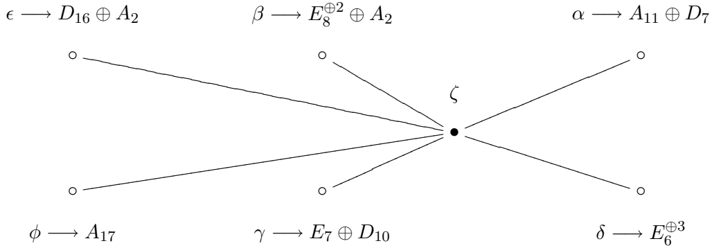
FIGURE 2. Matching of GIT and Baily–Borel boundary components
