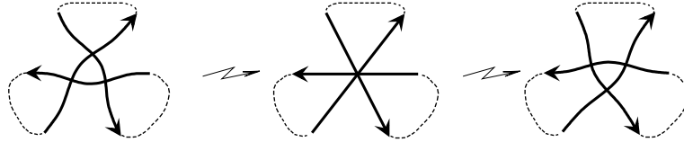
FIGURE 3. Triple point perestroika. Dotted curves indicate the scheme of connection of the branches, which is needed to determine the positive direction of the perestroika. On the right hand side q = 0 , on the left hand side q = 3 , thus the positive direction is to the right.
