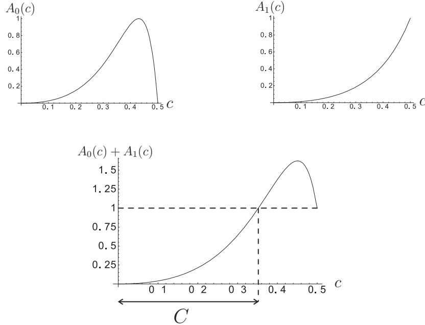
Figure 2.5: The graphs of A_0 , A_1 and A_0 + A_1
