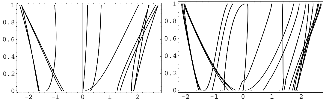
Figure 4.10: projection of periodic orbit 13 and 21 with Fibonacci combinatorics
