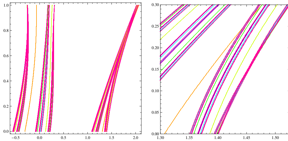
Figure 4.8: projection of periodic orbit 2^6 on x - plane
