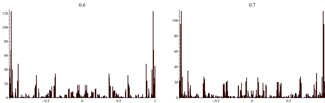
Figure 4.26: for the parameters (a, b) = \{(2.721829067829454, 0.6), (3.031843160671423, 0.7)\}
