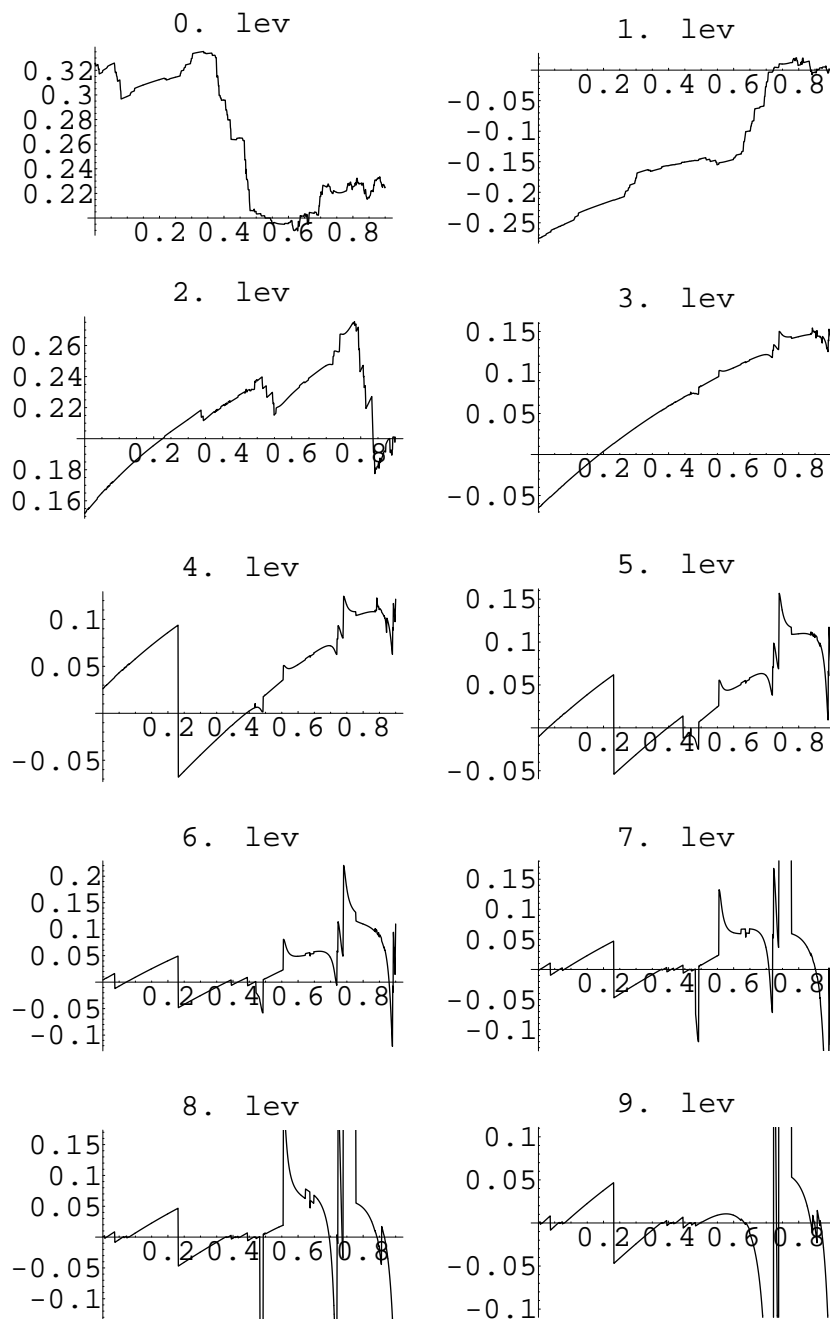
Figure 4.34: b versus average for downward angles; “ n lev” indicates the n th zoom level around the point l_p ;
