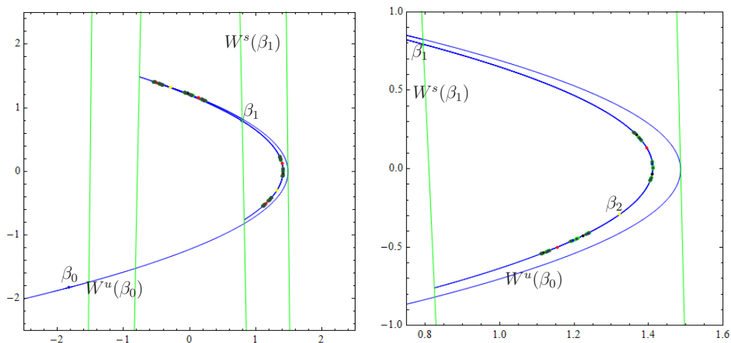
Figure 4.15: first heteroclinic tangency at b_1 ; \beta_0, \beta_1 are fixed points; W^u(\beta_0) is unstable manifold of \beta_0 and W^s(\beta_1) is the stable manifold of \beta_1 .
