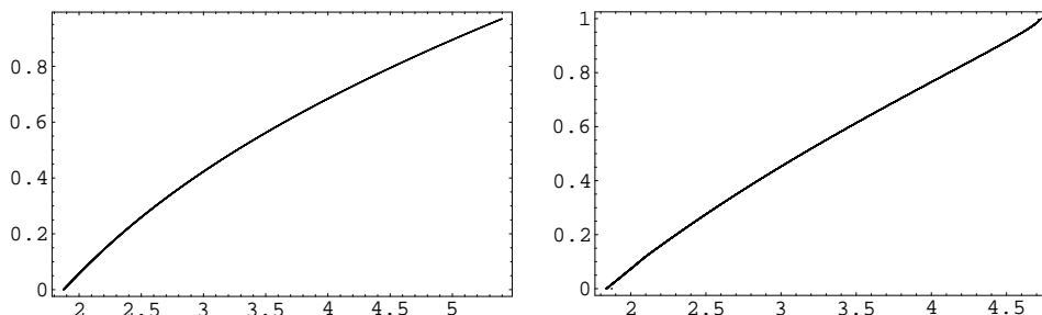
Figure 4.5: Fibonacci parameter curves of periods 13 and 21
