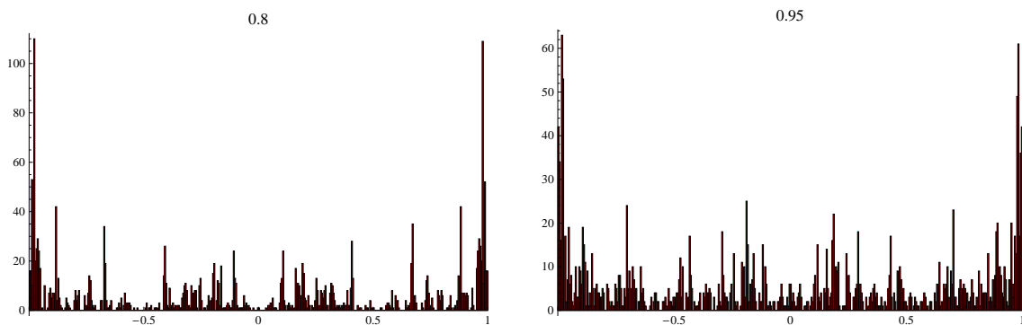
Figure 4.27: for the parameters (a, b) = \{(3.370236565105158, 0.8), (3.933243998542534, 0.95)\}
