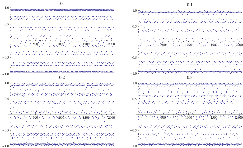
Figure 4.29: time versus angle for b = 0.0 to b = 0.3
