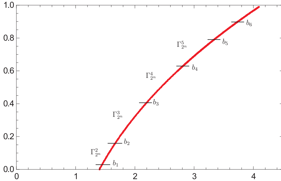
Figure 4.14: the curve \Gamma_{2^n}
