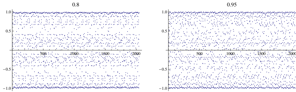
Figure 4.31: time versus angle for b = 0.8 and b = 0.95
