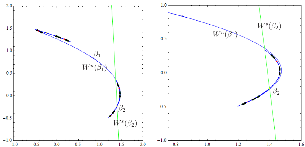
Figure 4.16: second heteroclinic tangency at b_2 ; \beta_1 is a fixed point and \beta_2 is period 2 point; W^u(\beta_1) is unstable manifold of \beta_1 and W^s(\beta_2) is the stable manifold of \beta_2 .
