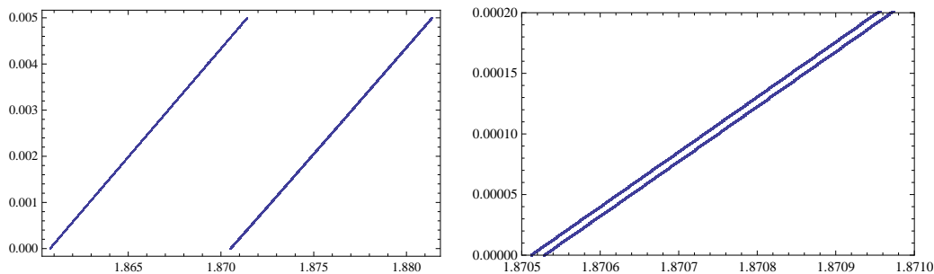
Figure 4.7: Left: period 5, 13 and 34; Right: Magnification of period 13 and 34
