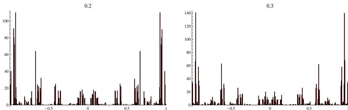
Figure 4.24: for the parameters (a, b) = \{(1.744828106932014, 0.2), (1.951646371711716, 0.3)\}
