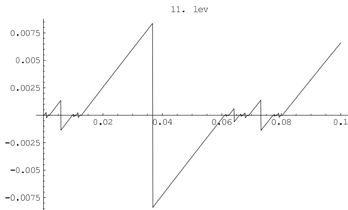
Figure 4.35: b versus average for downward angles
