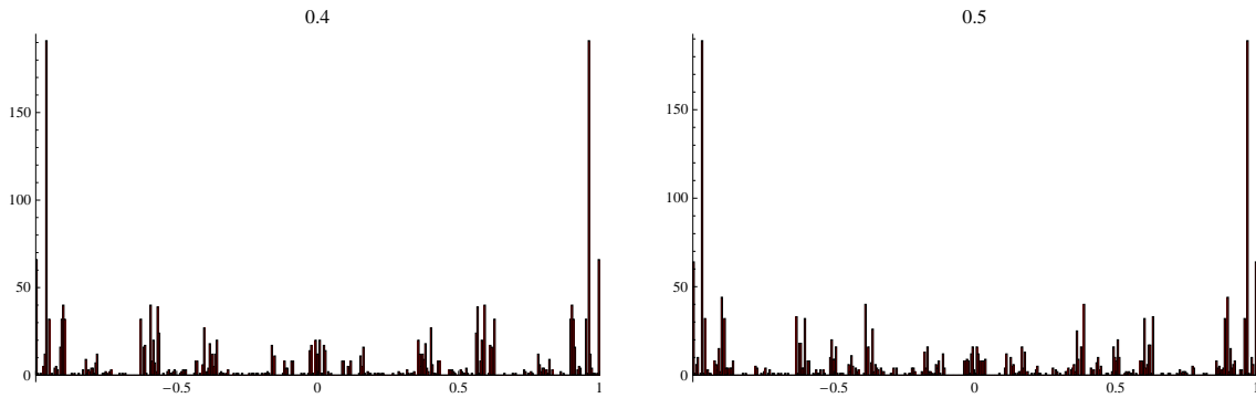
Figure 4.25: for the parameters (a, b) = \{(2.182768010790645, 0.4), (2.439153110310706, 0.5)\}
