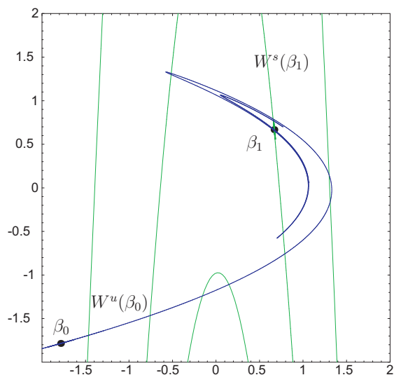
Figure 4.13: Non 2– renormalizable Hénon-like map
