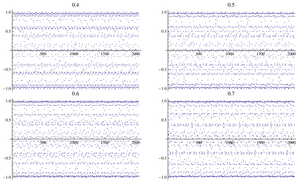
Figure 4.30: time versus angle for b = 0.4 to b = 0.7
