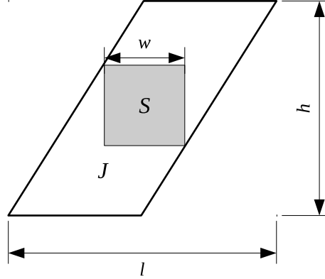
Figure 11.1.: The horizontal size l , the vertical size h , and the thickness w of a set J . In this picture, S is a largest square subset of J .
