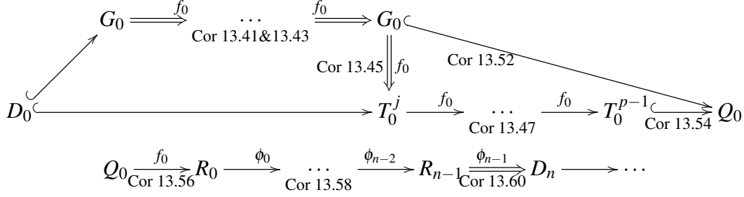
Figure 13.1.: A summary of all expansion estimates. The arrow \rightarrow represents expansion and the arrow \Rightarrow represents uniform expansion.
