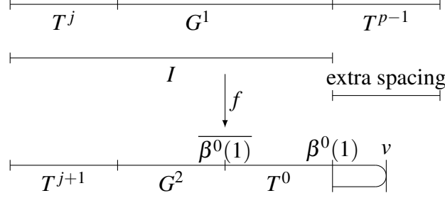
Figure 13.2.: The case of G \xrightarrow{f} G when T^{p-1} is adjacent to one of the boundaries.
