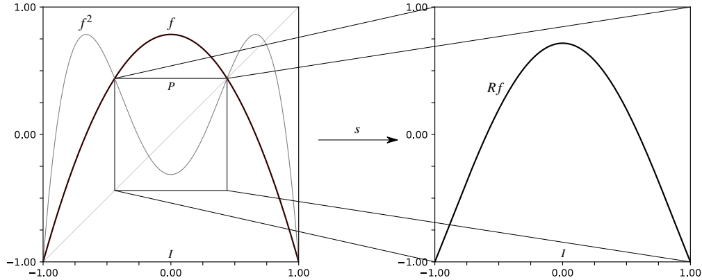
Figure 1.2.: A period-doubling renormalizable unimodal map f and its renormalization Rf .
