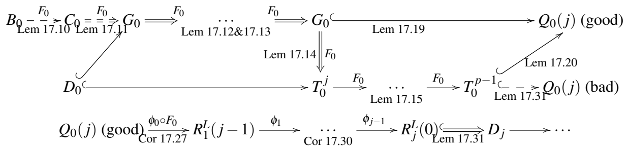
Figure 17.1.: A summary of all expansion estimates. The arrow \rightarrow represents expansion and the arrow \Rightarrow represents uniform expansion. The dash arrows are the paths addition to the unimodal case (compare Figure 13.1).
