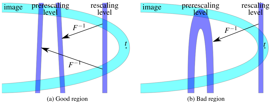
Figure 15.1.: Topology of the good region and the bad region
