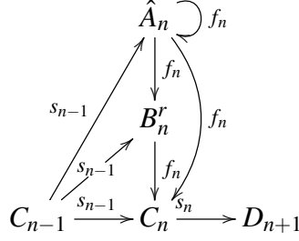
Figure 4.1.: Itinerary for a sequence of wandering interval.
