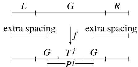
Figure 13.4.: The case G \rightarrow T^j .
