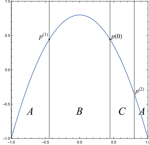
Figure 4.1.: The partition \{A, B, C\} of a unimodal map. The parabola is the graph of a unimodal map. The points p(0) , p(1) , and p(2) are defined as in Definition 4.4.
