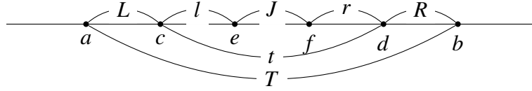
Figure 2.2.: Definition of the intervals T , t , L , l , R , r , and J .
