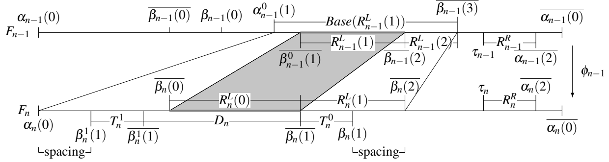
Figure 17.1.: The rescaling of the last step from R to D .
