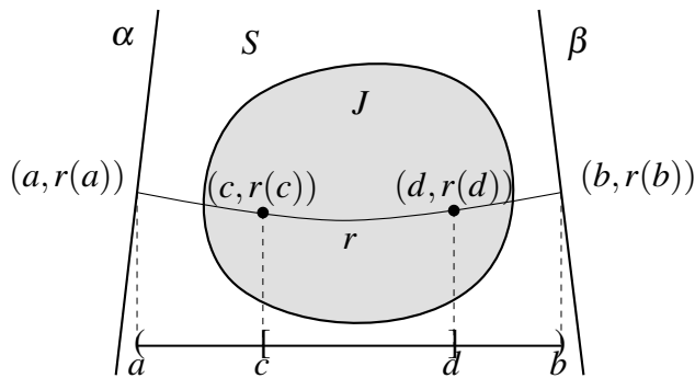
Figure 16.1.: Hyperbolic size measured by regular curves.
