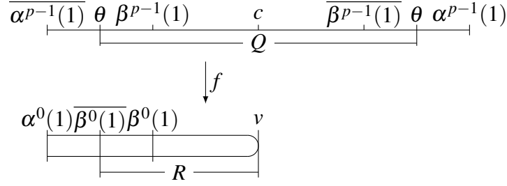
Figure 13.5.: The case Q \rightarrow R .
