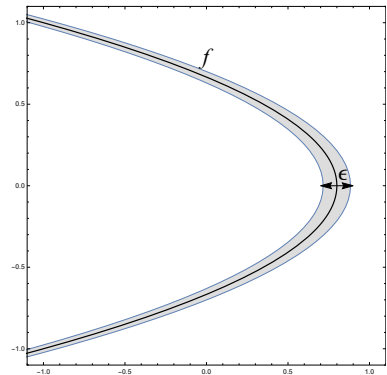
Figure 1.1.: The image of a Hénon map.
