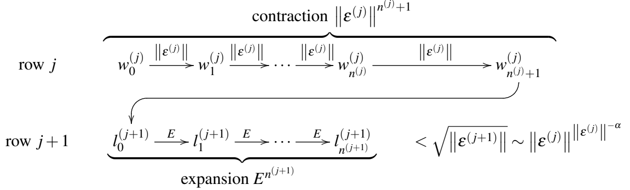
Figure 11.1.: The contraction, the expansion, and the sizes of the elements in the j -th and the (j+1) -th rows.
