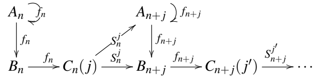
Figure 4.1.: The dynamics on the partition of a unimodal map.
