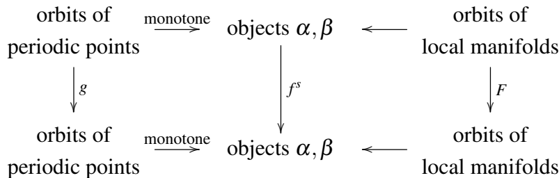
Figure 14.1.: The relation between the unimodal map, induced unimodal map, and the Hénon-like map.
