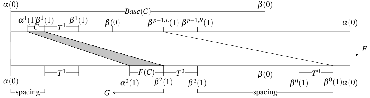
Figure 17.2.: The iteration from C to G .
