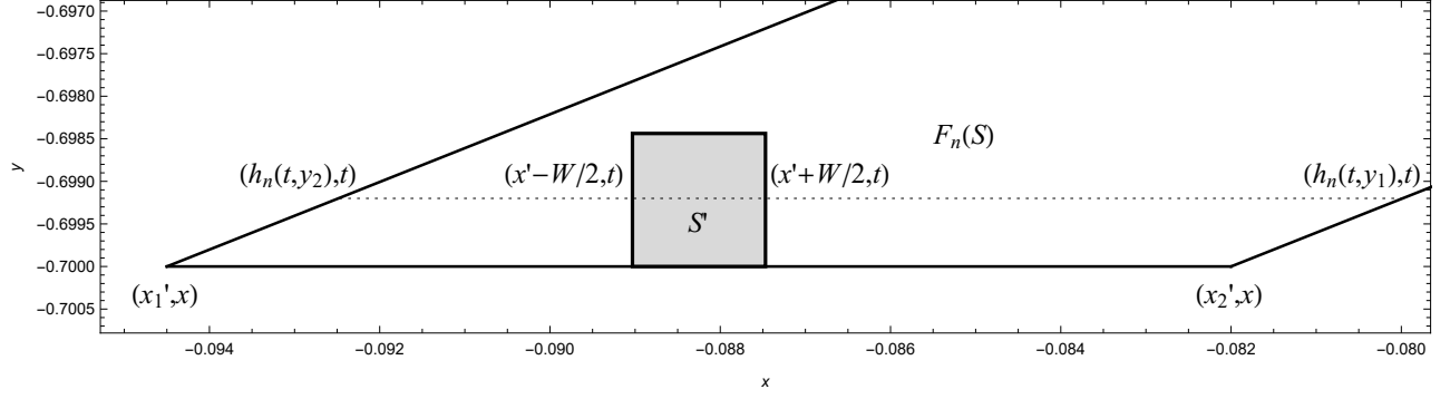
Figure 11.2.: Four points on the cross section y = t .
