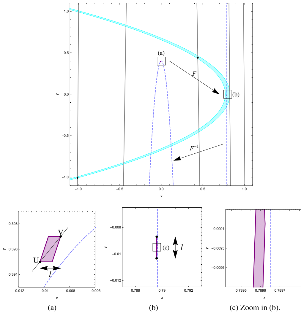
Figure 9.1.: The vertical line argument. The scales of the graphs in (a) and (b) are the same.
