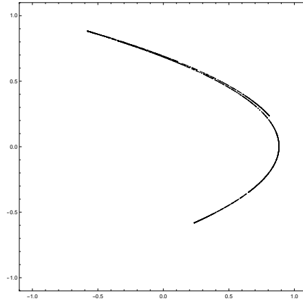
(b) A Hénon map that is not period-doubling renormalizable.
