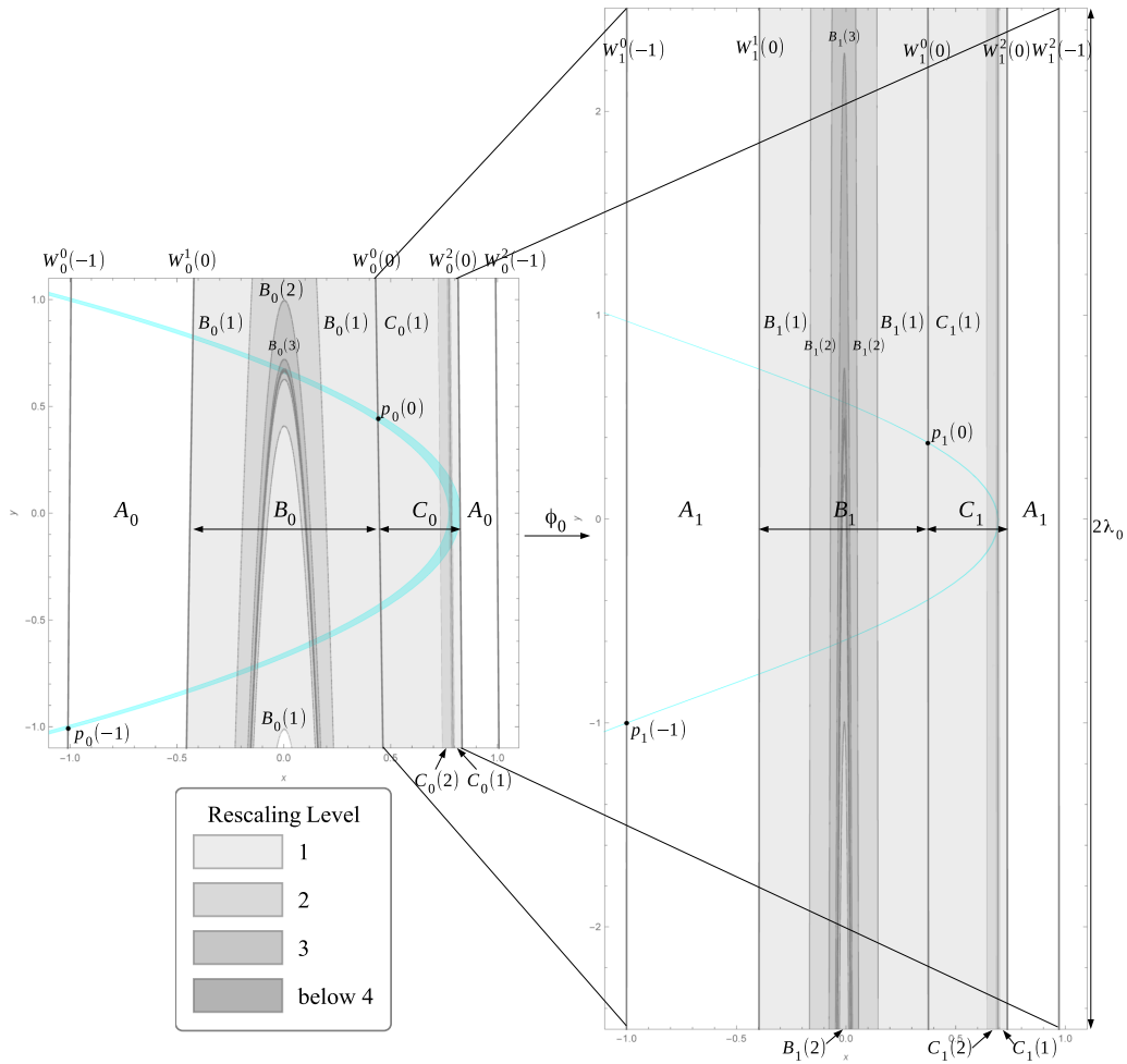
Figure 6.1.: The partition and the local stable manifolds of two renormalization scales F_0 and F_1 from the left to the right. The rescaling levels 1, 2, 3, and below 4 are shaded from light to dark as shown in the legend.
