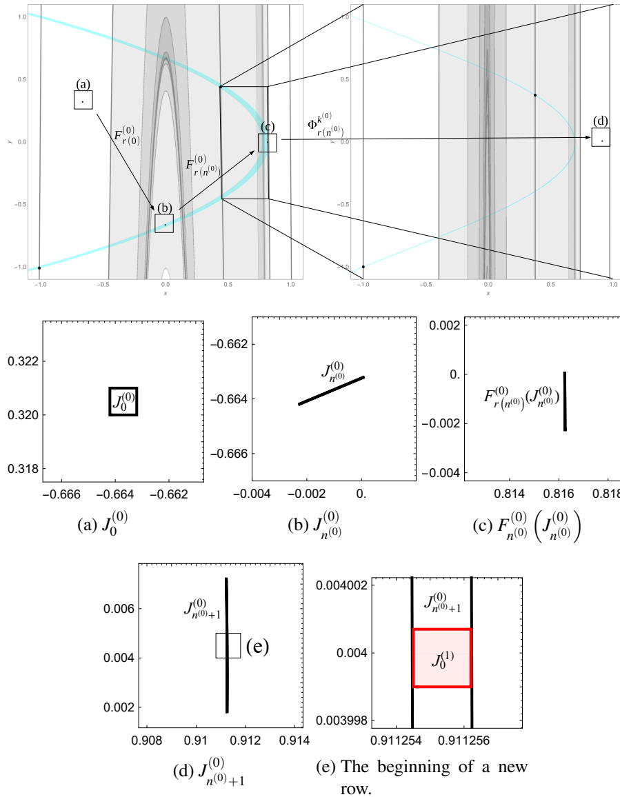
Figure 11.2.: An example of a double sequence. The graphs are the domains of F_0^{(0)} and F_1^{(0)} = F_0^{(1)} from the left to the right. The arrows indicate an iteration or a rescaling from one element to the other one. The sub-figures (a), (b), (c), (d), and (e) are elements of the double sequence in a zoomed scale. The scales of (a), (b), (c), and (d) are the same.
