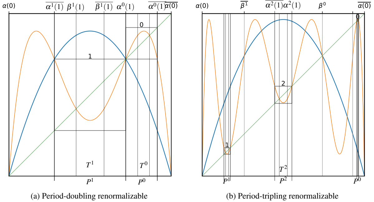
Figure 13.1.: The cyclic intervals of renormalizable unimodal maps
