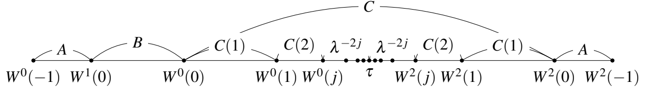
Figure 6.1.: The structure of the rescaling levels. The figure shows the partition and the local stable manifolds on the horizontal cross section that intersects the tip.
