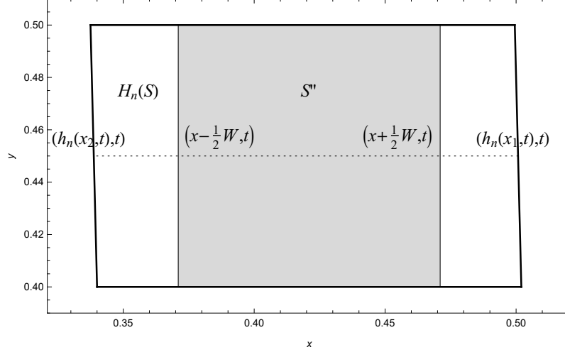
Figure 11.3.: Four points on the cross section y = t .
