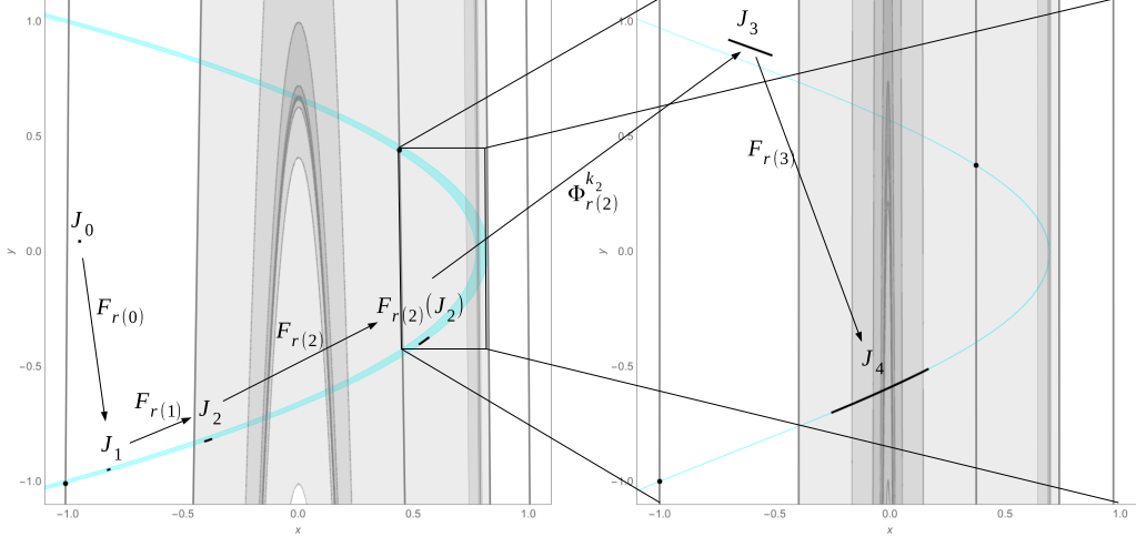
Figure 7.1.: The construction of a closest approach J_n . The graphs are the domains and the partitions of F_0 and F_1 from the left to the right.
