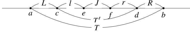
Figure 4.2.: Definition of T , T' , L , l , R , r , and J .
