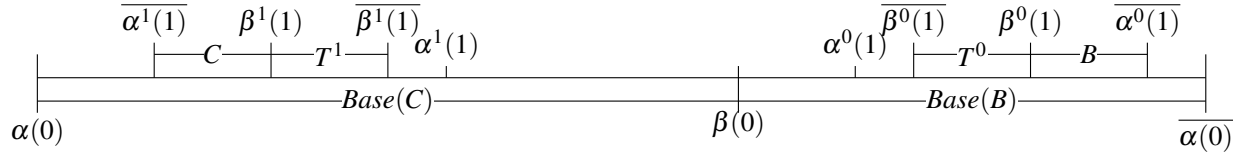
Figure 17.1.: The iteration from B to C .
