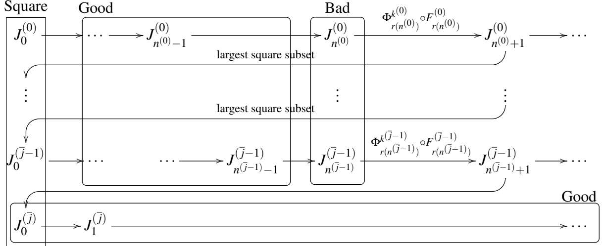
Figure 11.1.: The construction of a double sequence.
