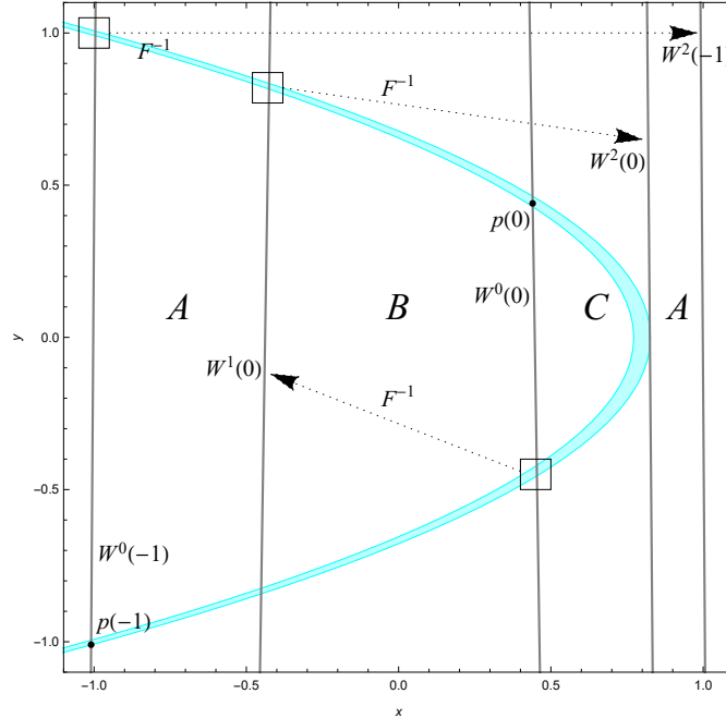
Figure 5.1.: Local stable manifolds and the partition of a Hénon-like map F . The shaded area is the image of the Hénon-like map. The vertical graphs are the local stable manifolds W^0(-1) , W^1(0) , W^0(0) , W^2(0) , and W^2(-1) from left to right. The arrows illustrates the construction of each local stable manifold.
