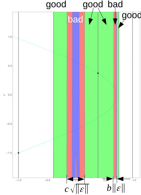
Figure 9.2.: The good region and the bad region. The rescaling levels 1, 2, and below are the shaded area colored from light to dark. In this example, one can see a tiny light area on the center bottom part of the graph. This is because C^r(2) intersects the image F(D) . Hence, the boundary is K = 2 and the good region contains the lightest part and the bad region contains the two darker parts.
