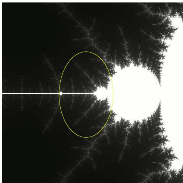
Figure 5.4.2: A computer approximation of the M -set of fix on \mathcal{W}^u(fix) . The restricted M -set used in the Estimating Lemma is contained in the ellipse which is included for illustrative purposes only.
