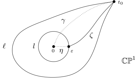
Figure 2.3: Deforming the loop l
