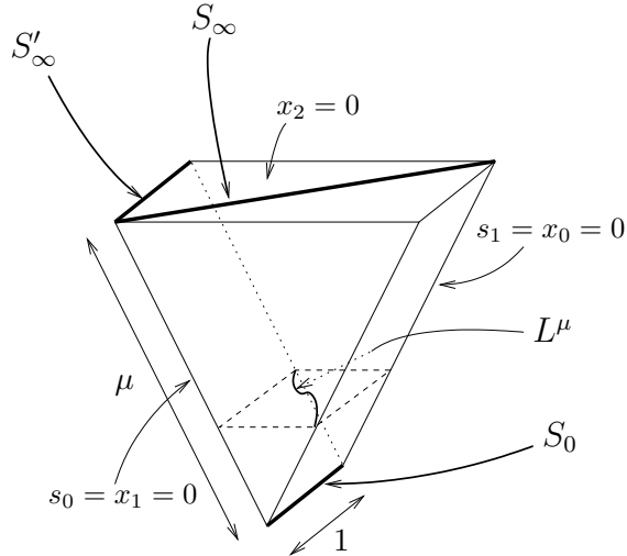
Figure 4.1: Polytope representing (\mathbb{C}\mathbb{P}^1 \times \mathbb{C}\mathbb{P}^2, \sigma_\mu)
