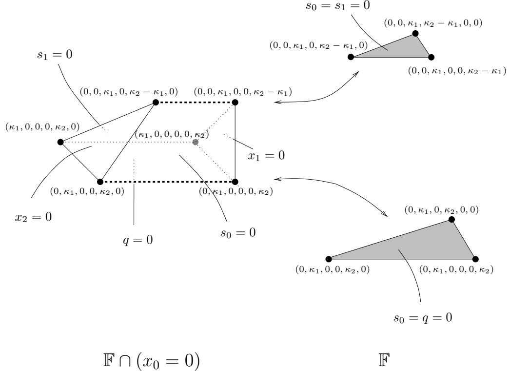
Figure 3.2: Polytope \Delta^\kappa representing (\mathbb{F}, \omega_{\mathbb{F}}^\kappa) for n = 1
