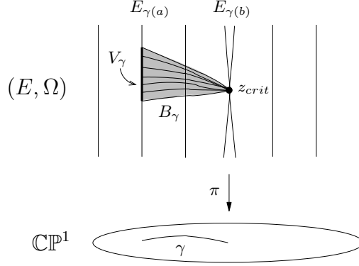
Figure 2.2: The vanishing cycle
