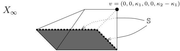
Figure 3.4: X_\infty in \mathbb{F} \cap (x_0 = 0)
