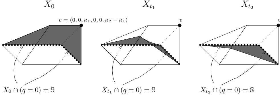
Figure 3.3: X_t in \mathbb{F} \cap (x_0 = 0)
