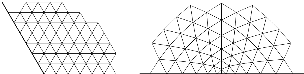
FIGURE 8. Near the 120^\circ corner, the conformal map acts like a power map z \rightarrow z^{3/2} . The image triangulation contains two 90^\circ angles.
