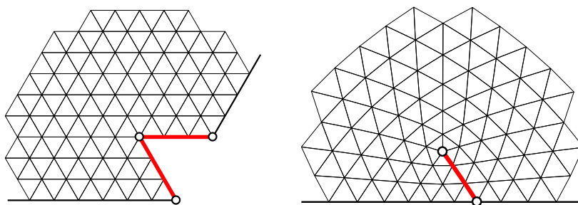
FIGURE 9. The “120°-trick” from [9] creates a triangulation of a half-plane with maximum angle 72^\circ (right side) by taking the conformal image of an equilateral triangulation of a 120^\circ -sector with some triangles removed (left side). Two boundary arcs on the modified sector are identified as one internal arc \gamma in the new triangulation, and an interior vertex of degree 5 is created. The arc \gamma appears straight, but is actually slightly curved to ensure the image vertices on either side of \gamma match up (that this is possible is proved in [9]). The conformal map approximates z^{3/2} near infinity, hence the new triangulation approximates the z^{3/2} -triangulation from Figure 8 near infinity.
