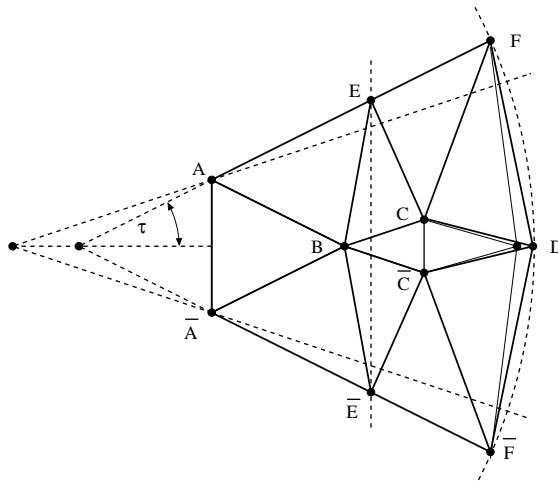
FIGURE 16. This is the same as Figure 15, except that D has been moved to the right, so the region becomes a polygonal sector. Only the angles of triangles containing D are changed, and all change monotonely.
