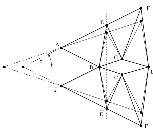
FIGURE 15. The first variation. We move the vertices E, \bar{E}, F, \bar{F} in Figure 12 vertically so that they lie on a new line making a larger angle with the horizontal. The other points are not moved. Every angle changes monotonely. Since D is not moved, the new figure is not quite a polygonal sector. This is fixed in Figure 16.
