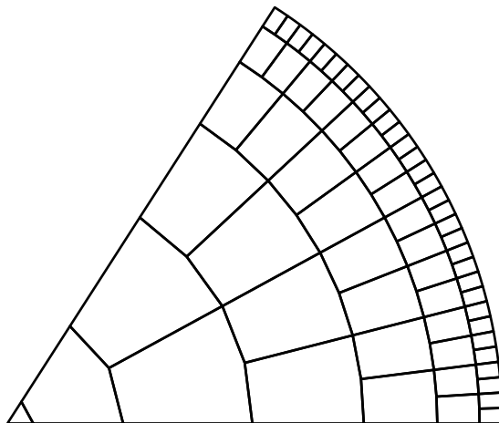
FIGURE 11. A mesh of a polygonal sector into one triangle and several pentagons.
