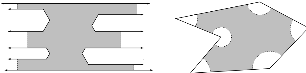
FIGURE 2. We use the conformal map to transfer a nearly equilateral triangulation from a compact region of the model domain (shaded) to the interior of P minus neighborhoods of each vertex. We then have to triangulate the neighborhoods and make the meshes match up.
