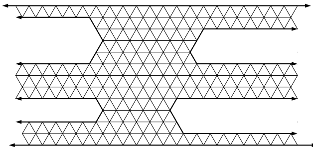
FIGURE 1. A model domain is a subset of an infinite strip that has four closed regions removed. Each closed region is bounded by an unbounded Jordan curve consisting of two horizontal infinite rays and two finite segments and has three angles of 120^\circ . In this figure, the model domain has an equilateral triangulation, although most model domains only have nearly equilateral triangulations (see Lemma 2.1). In this picture there are six infinite ends: three go left, three go right, and there are two ends each of thicknesses 1, 2 and 3.
