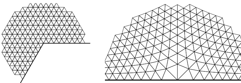
FIGURE 4. Mapping an equilateral triangulation of a 240^\circ sector by z \rightarrow z^{3/4} gives a 67.5^\circ -triangulation. The maximum occurs in the four triangles touching the origin.
