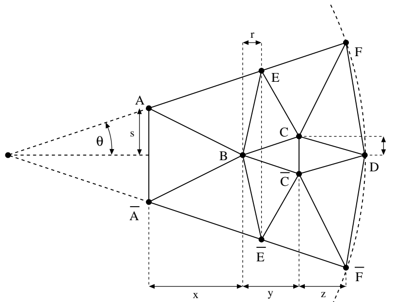
FIGURE 12. The triangulation \mathcal{T}(\theta) of a polygonal sector. The precise definition is given in the text. We assume 0 \leq \theta \leq 30^\circ .
