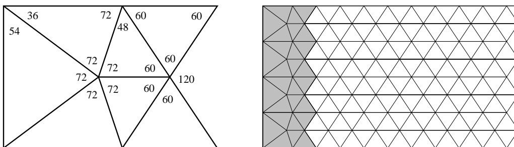
FIGURE 6. On the left is a triangulation of an indented rectangle. Note that every angle is \leq 72^\circ . On the right we show how it “fills in” between a partial equilateral triangulation of strip and the end of a half-strip.
