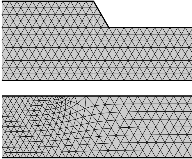
FIGURE 7. We use a conformal map to transfer equilateral triangulation from a “funnel strip” to a true strip. Enlargements of the behavior near the 120^\circ and 240^\circ corners are illustrated on Figures 4 and 8. These figures were produced with Driscoll’s SC-Toolbox [14].
