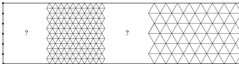
FIGURE 5. Two problems involved with merging the triangulations. On the left we have to complete the triangulation between an equilateral triangulation and the end of a half-strip. On right we have to interpolate between two equilateral triangulations of different sizes. In our applications, we are free to choose the widths of the intermediate regions to be meshed.
