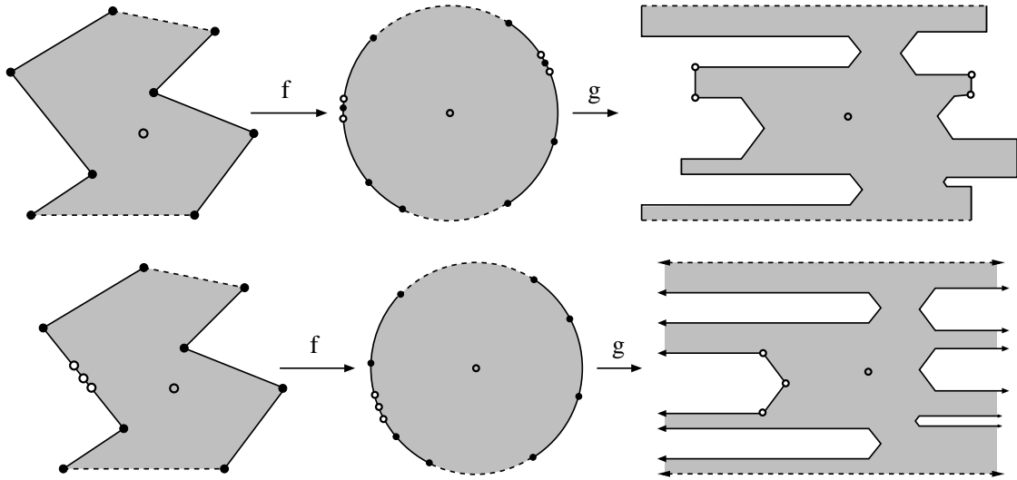
FIGURE 3. Using the Schwarz-Christoffel formula, one can map the interior of any simple polygon to a subset of a strip as shown on top. By taking the preimages z_k^\pm of the 90^\circ corners to converge to z_k , we get a conformal map onto an unbounded model domain, as shown on the bottom.
