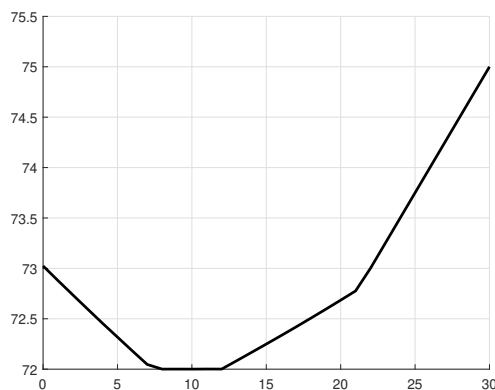
FIGURE 13. The maximum angle used in the triangulation \mathcal{T}(\theta) for 0 \leq \theta \leq 30^\circ based on a computerized search for parameters. This indicates the estimate \leq 75^\circ is true with the maximum attained at 30^\circ .
