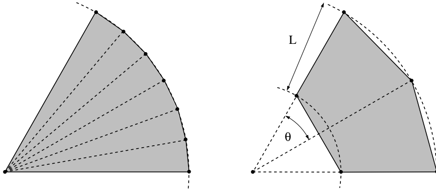
FIGURE 10. On the left is a general polygonal sector. On the right is a truncated polygonal sector; in this case a pentagon, the case of greatest interest to us. We want to triangulate such pentagons with good angle bounds without adding any vertices to the “inner” and “outer” sides.
