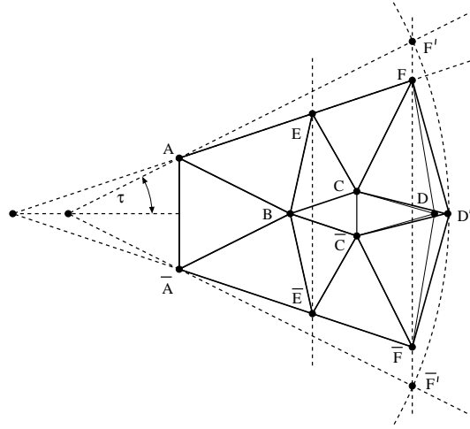
FIGURE 17. This is the second variation: we move D but not E or F . As we move D , all the angles of triangles containing D change monotonely. To make this a polygonal sector, we then have to move E, F and their conjugates vertically.
