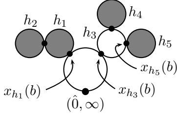
Figure 3: An Example of the Estimates (4.14) and (4.15)
