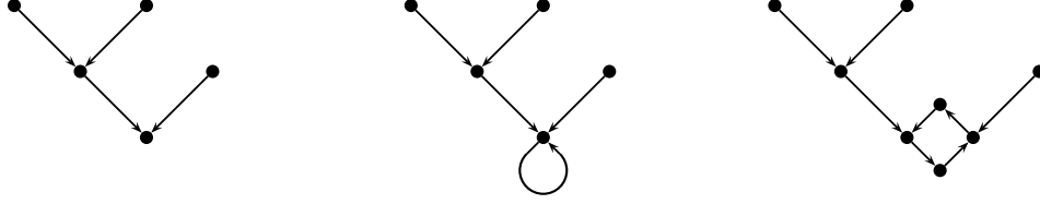
Figure 2: Some Enhanced Linearly Ordered Sets
