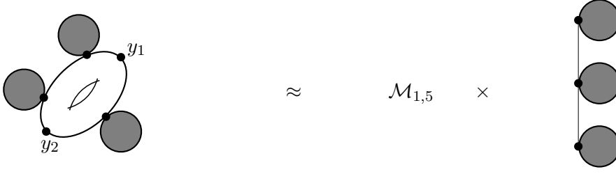
Figure 5: An example of the decomposition (3.17)
