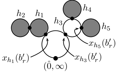
Figure 4: An example of the estimates (2.7) and (2.8)
