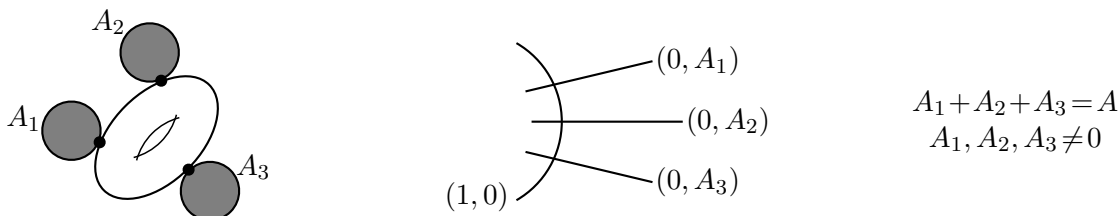
Figure 1: The domain of an element of \mathfrak{M}_{1,k}^3(X, A; J)
