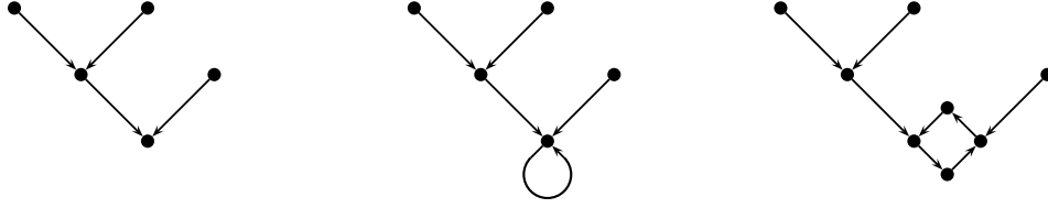
Figure 3: Some enhanced linearly ordered sets
