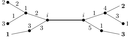
Figure 3: A graph representing a fixed locus in \mathfrak{X}_d ; i \neq 1, 3, 4
