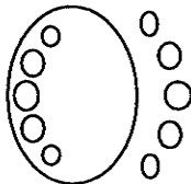
Figure 5. Real scheme of Gudkov's curve of degree 6.
