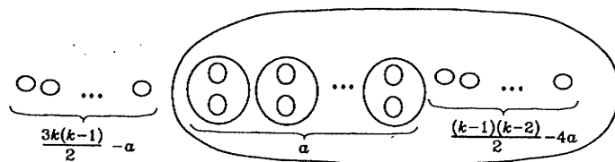
Figure 12. Real scheme of a curve of degree 2k with p = 3k(k - 1)/2 + 1 + a .
