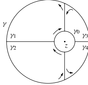
FIGURE B.4. Computation of \int_{\gamma} (\zeta - z)^{-1} d\zeta over a standard circle when z is not the center.
