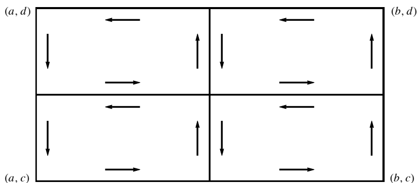
FIGURE B.1. First bisection of the rectangle R in Goursat's Lemma.
