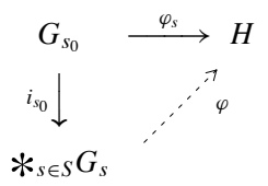
FIGURE 7.2. Universal mapping property of a free product.
